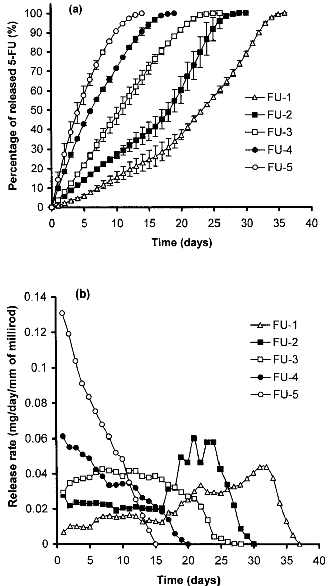
Figure 4. Cumulative release (a) and rate profiles (b) of membrane-encased millirods. The structural composition for each type of millirod is listed in Table I. The error bars in Figure 4(a) were measured from triplicate samples. For clarity of presentation, the error bars were not shown in Figure 4(b).
