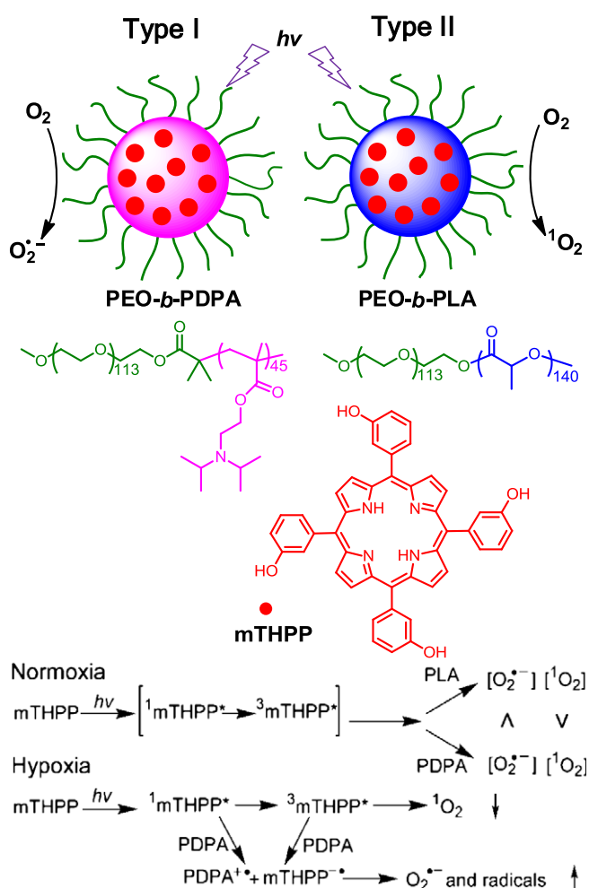
Scheme 1. Modulation of photoactivation mechanism of a model photosensitizer, mTHPP, by the micelle microenvironment at normoxic (~50 mm Hg \text{O}_2 ) and hypoxic (<20 mm Hg) conditions. Electron-rich PDPA micelles led to increased type I reactions producing superoxide radical anions, while electron-deficient PLA micelles generated singlet oxygen as predominant species by type II reactions.
