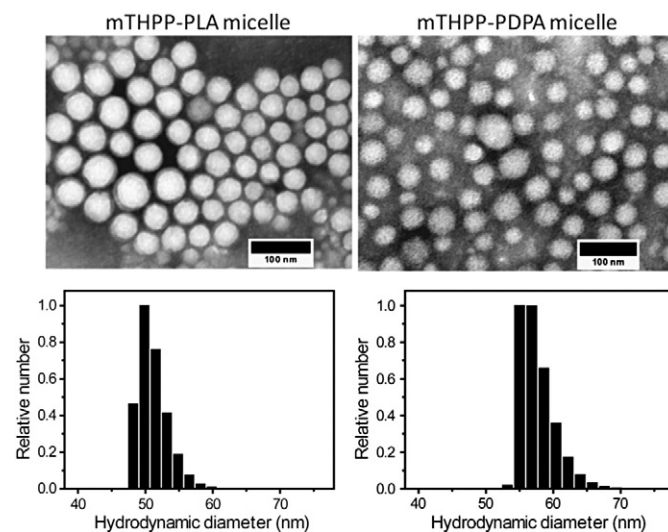
Fig. 1. Transmission electron microscopy (TEM) images of mTHPP-loaded micelles counter-stained with 2% phosphotungstic acid. The scale bars are 100 nm. Histograms depict hydrodynamic diameter distributions of mTHPP-loaded micelles by dynamic light scattering (DLS).
