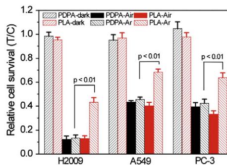
Fig. 4. Relative survival of different cancer cells irradiated with 12 \text{ J/cm}^2 (power density 20 \text{ mW/cm}^2 ) of 532 nm light in atmospheres of air and argon. Micelle concentration: 200 \mu\text{g/ml} . Incubation time: 2 h. Values represent treat/control (T/C) \pm standard deviation ( N = 6 ).
