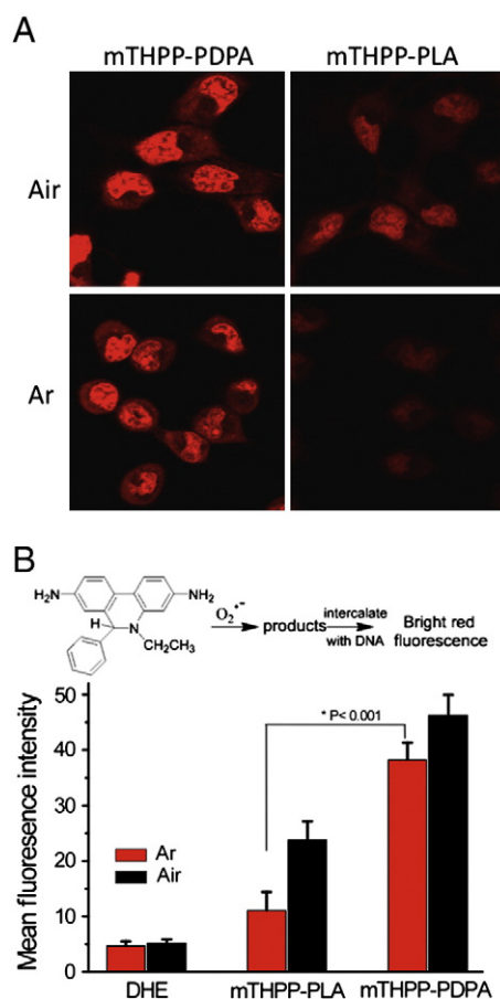
Fig. 3. (A) Confocal laser scanning microscopy images of H2009 lung cancer cells after incubation with 150 \mu\text{g/ml} mTHPP micelles for 2 h, followed by incubation with DHE for 30 min in air or argon-saturated PBS, then irradiated with 532 nm laser light at 20 \text{ mW/cm}^2 for 4 min. (B) Average fluorescence intensity from 10 cells calculated by ImageJ for different treatment groups. H2009 cells without mTHPP micelle treatment, but incubated with DHE were used as the control (DHE).
