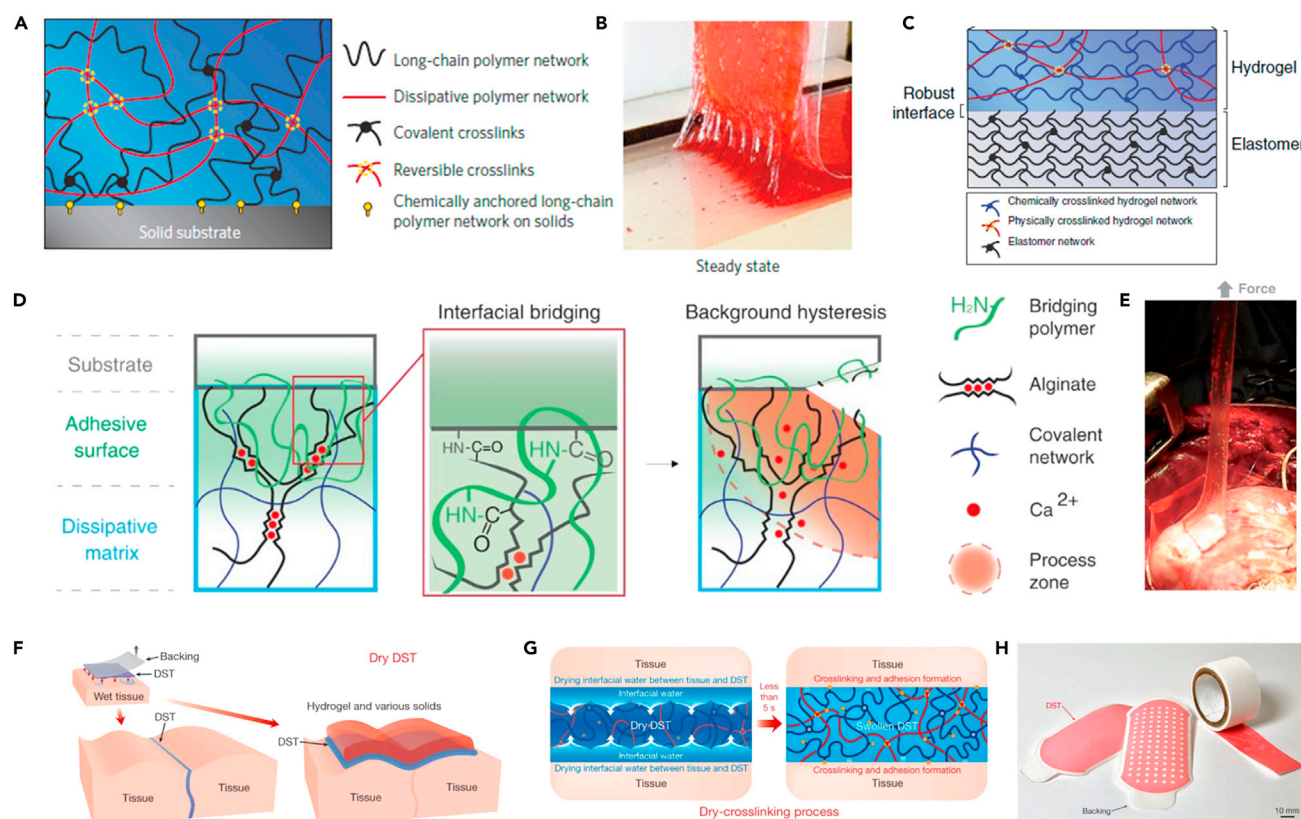
Figure 5. Hydrogel adhesives
